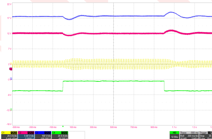
Figure 5: Load transient with 600µF hold-up capacitor (50%-75%-50% of I_{max} , 115Vrms, 60Hz) Ch1: I_{in} (20A/div), Ch2: V_{out} (5V/div), Ch3: Hold-up capacitor voltage (100V/div), Ch4: I_{out} (20A/div), Timebase: (200ms/div).
