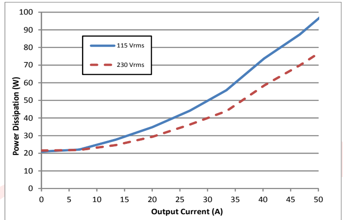
Figure 2: Power dissipation at nominal output voltage vs. output current for 115Vrms and 230Vrms input voltage (applies to both 60Hz and 400Hz) at T_b =
