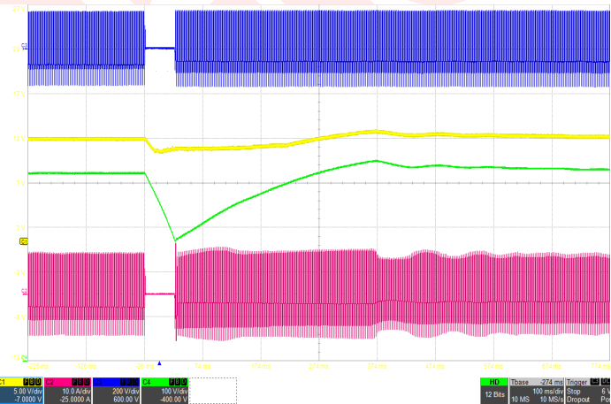
Figure 10: Line drop out with 600µF hold-up capacitor at full load (115Vrms, 400Hz) Ch1: Vout (5V/div), Ch2: Iin (10A/div), Ch3: Vin (200V/div), Ch4: Vhold-up (100V/div), Timebase: (100ms/div).
