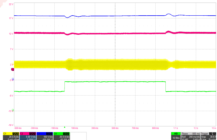
Figure 6: Load transient with 600µF hold-up capacitor (50%-75%-50% of I_{max} , 115Vrms, 400Hz) Ch1: I_{in} (20A/div), Ch2: V_{out} (5V/div), Ch3: Hold-up capacitor voltage (100V/div), Ch4: I_{out} (20A/div), Timebase: (200ms/div).
